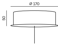
Canopy for PC1289, PC1290
