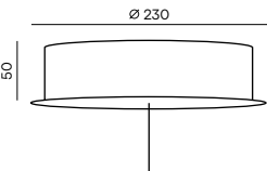
Canopy for PC1289, PC1290 for PWM dimming system
