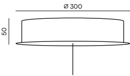
Canopy for PC1291 incl. PWM dimming system
